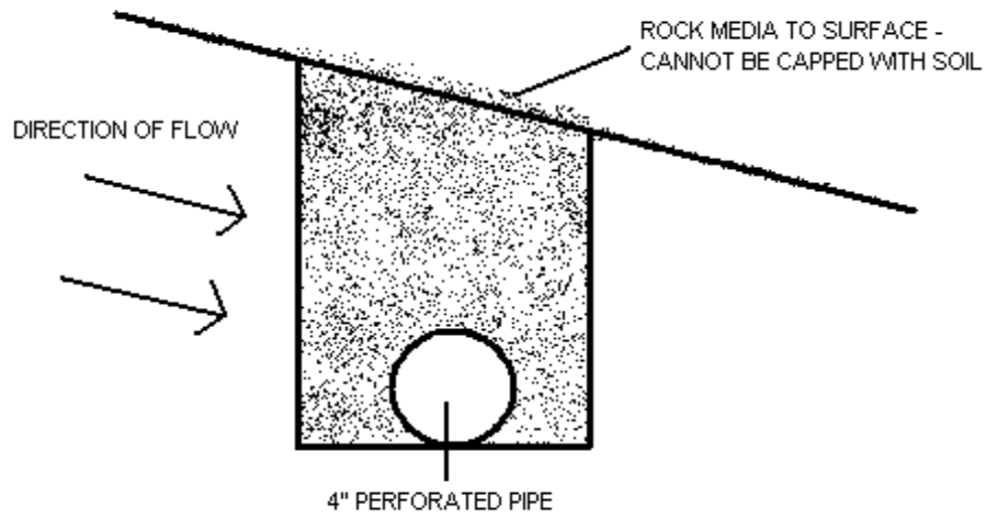
CURTAIN DRAIN CROSS-SECTION
